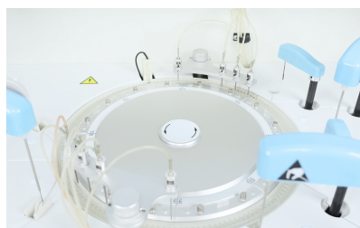
Reaction Tray 37±0.1°C. Water Bath.
